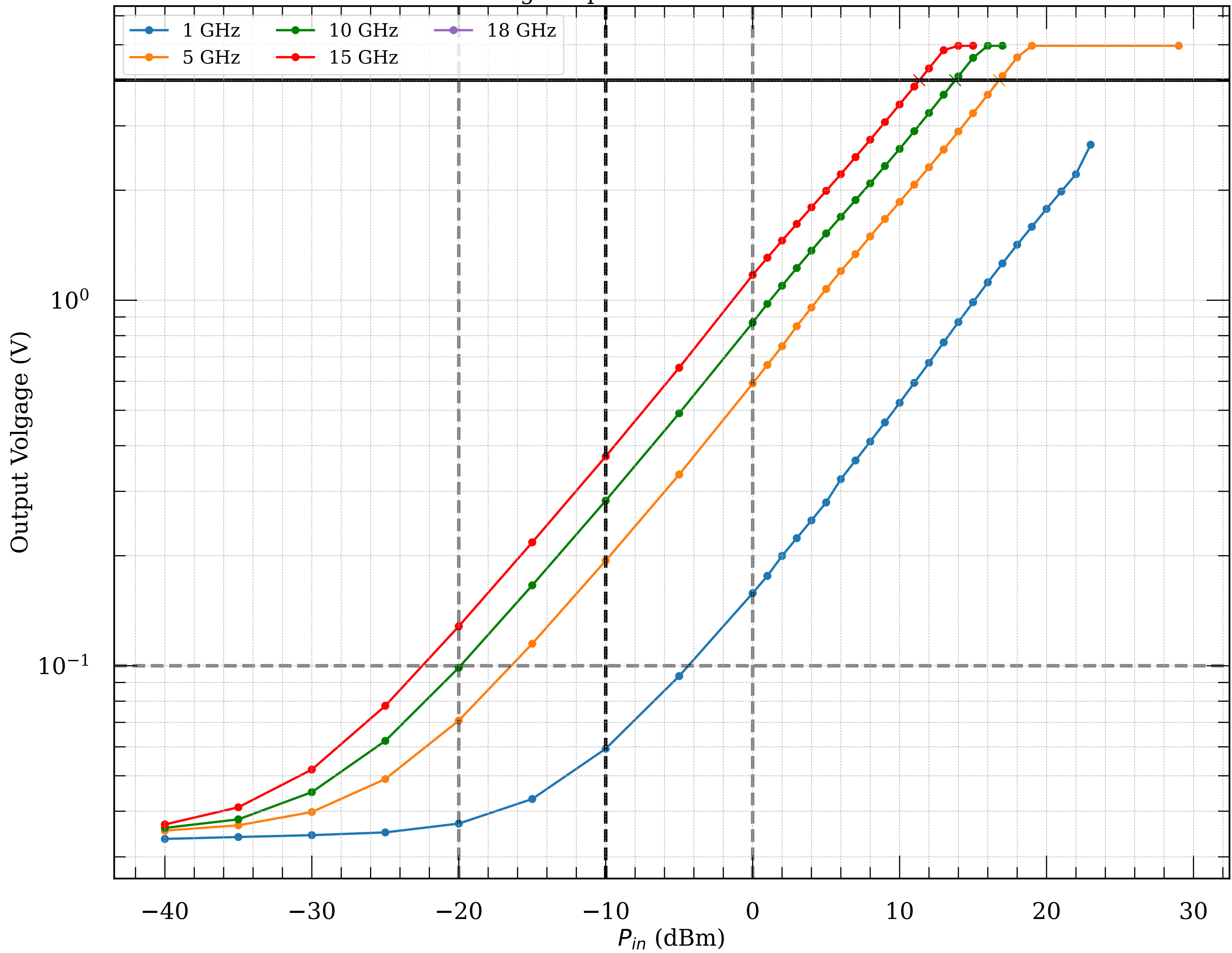
Measured voltage-to-power curve of detector module033
